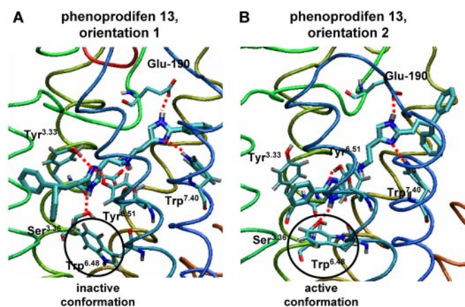
Fig. 4. Binding mode of phenoprodifen 13 at gpH 1 R. A, stable conformation of phenoprodifen 13 in the binding pocket of gpH 1 R, observed in MD simulations in orientation 1. B, stable conformation of phenoprodifen 13 in the binding pocket of gpH 1 R, observed in MD simulations in orientation 2. The MD-simulations were performed as described under Materials and Methods . Hydrogen bonds and electrostatic interaction between ligand and amino acids are marked as red dashed lines. At hH 1 R, binding modes of phenoprodifen 13 were similar to the modes at gpH 1 R. The amino acids of the transmembrane domains are numbered concerning to the nomenclature of Ballesteros et al. (2001).
