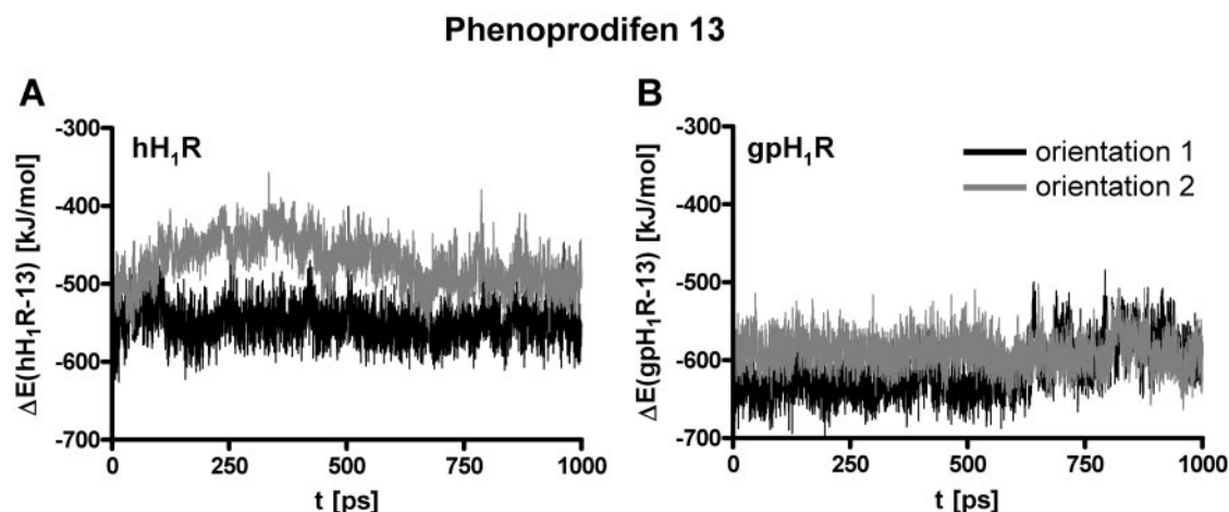
Fig. 5. Interaction energy of phenoprodifen 13 with hH 1 R and gpH 1 R in orientations 1 and 2. The interaction energy of phenoprodifen 13 with hH 1 R [ \Delta E(\text{hH}_1\text{R}-\mathbf{13}) ] and with gpH 1 R [ \Delta E(\text{gpH}_1\text{R}-\mathbf{13}) ] was calculated during a 1-ns productive phase in MD simulation. At each time step, the potential energy of the receptor and of the ligand were subtracted from the potential energy of the corresponding ligand receptor complex.
